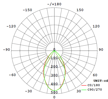
Diagram for RUL06X4-01 in 3000K Other diagrams available on request
