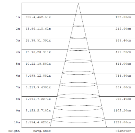
Diagram for RUL06X4-01 in 3000K Other diagrams available on request
